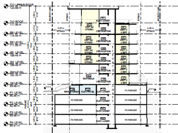
site section a
