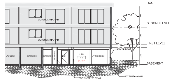
4 BUILDING 3 NEW SECTION A305 1/8"=1'-0"
