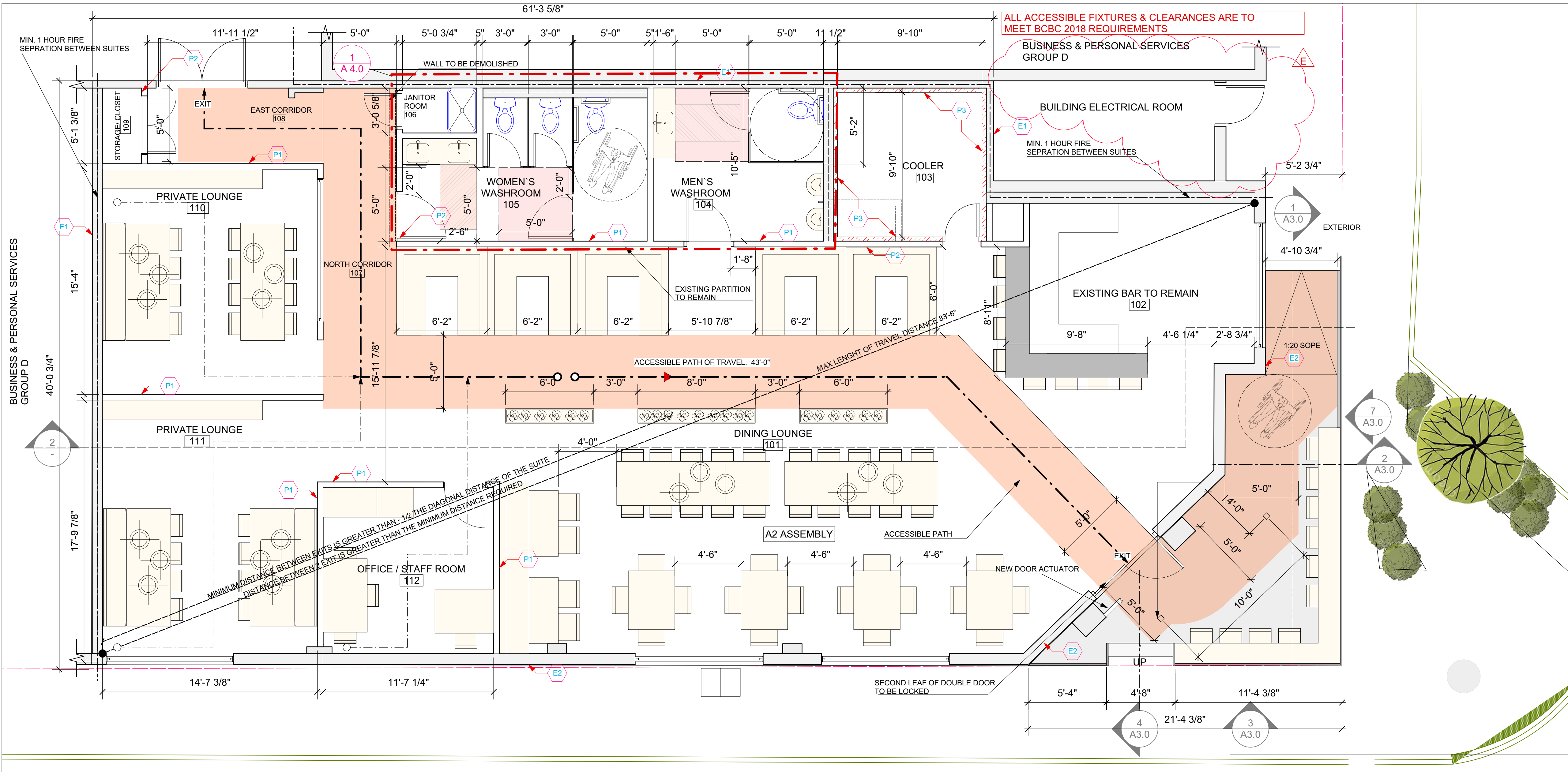
1 PROPOSED FLOOR PLAN A1.0 SCALE: 1/4" = 1'-0"
